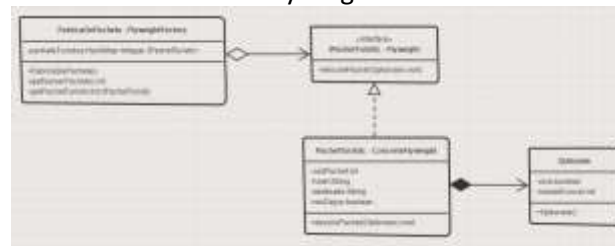
Flyweight
